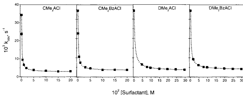
Figure 2. Dependence of observed rate constants, k_{\text{obs}} , on [surfactant] for cationic micelles at 35 °C. The points are experimental and the curves were calculated using Eqn. (1)
